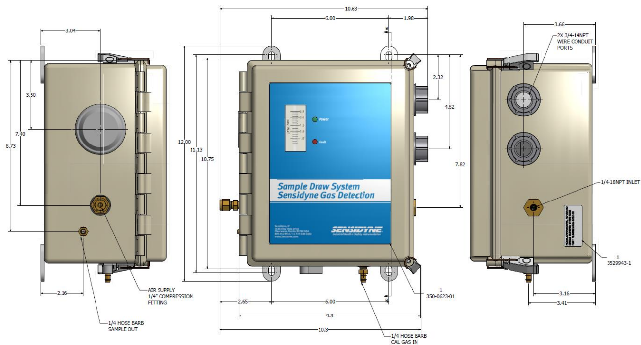
Figure 5 Dimensional Drawing
